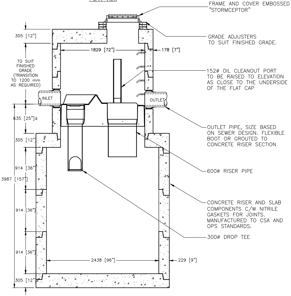
SECTION VIEW
