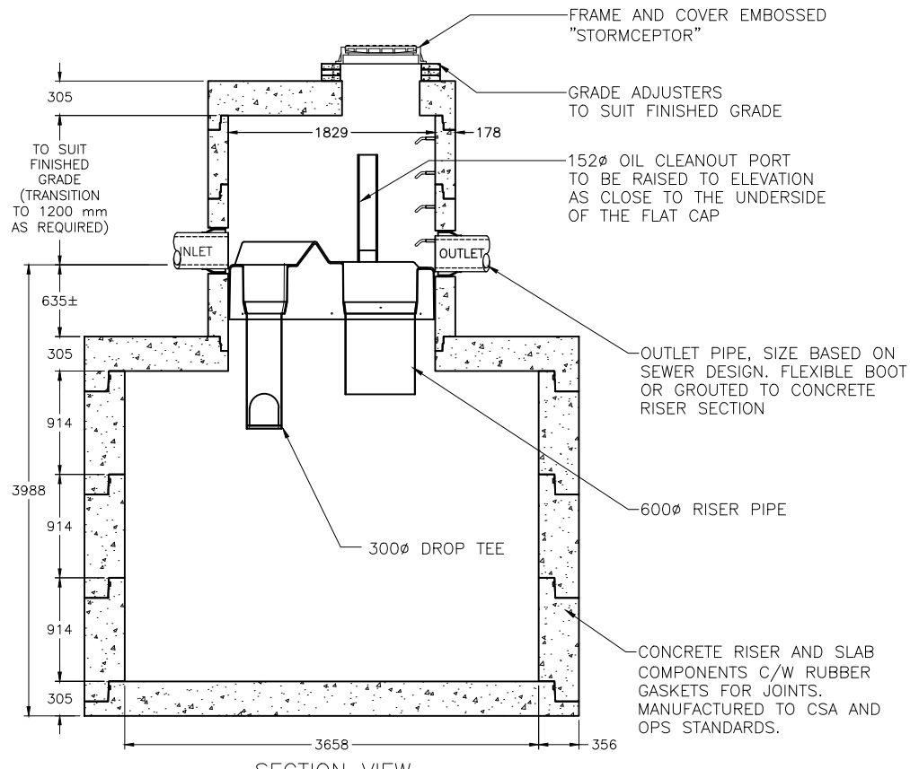
SECTION VIEW
